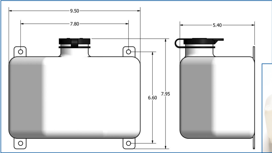
70 Oz. Bottle w/ Snap Cap Part No. 14-111211
