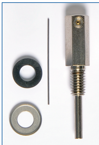
Part No. 14-004000 Single Jet Spray Nozzle 2.9"Lx1/2"D
