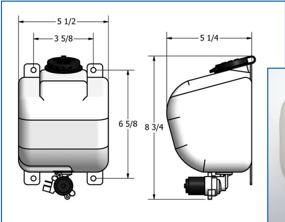
70 Oz. Bottle w/ Snap Cap Part No. 14-111211
